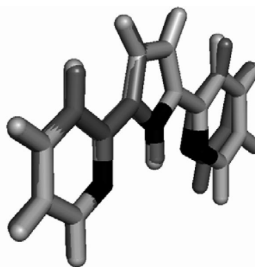
Figure 8. Superposition of the experimental (gray) and the theoretical (pale gray) structures of 2,5-dipyridin-2-ylpyrrole. An RMS deviation value of 0.044 Å was calculated by taking into account the two coplanar rings.
