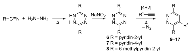
Scheme 2. Pyridazine synthetic pathway.
