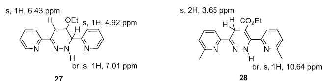
Figure 3. Dihydropyridazine derivatives obtained as a byproduct ( 27 ) or sole compound ( 28 ) of the electrochemical reduction run at the potential of the first reduction peak ( E_{p1} ) of the corresponding pyridazine 12 and 13 , respectively.
