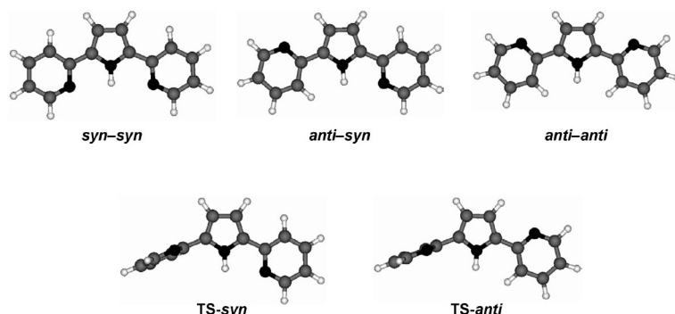
Figure 4. Minima and transition-state conformers of 2,5-dipyridin-2-ylpyrrole 18 found at the MPWB1K/6-31+G(d,p) level.
