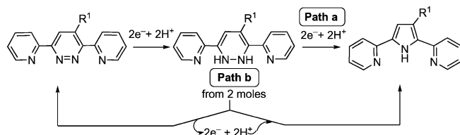
Scheme 3. General transformation pathway of pyridazines into pyrroles.
