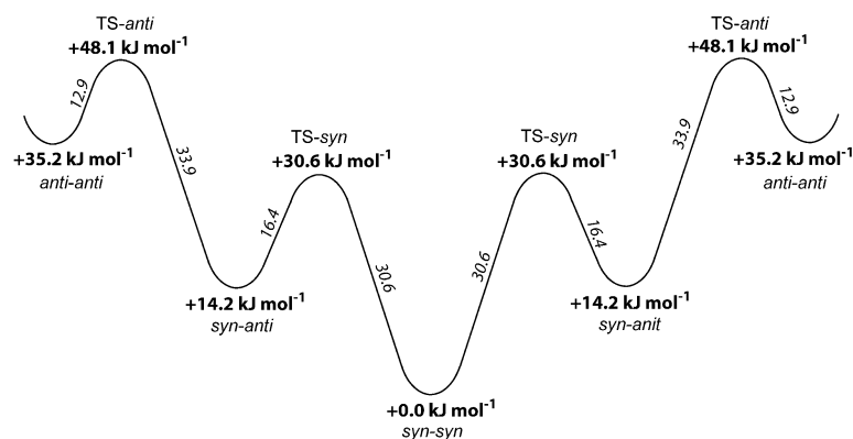
Figure 5. Conformational profile of 2,5-dipyridin-2-ylpyrrole 18 obtained at the LMP2/6-311++G(d,p)//MPWB1K/6-31+G(d,p) level with relative energies and rotation barriers.
