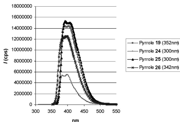
Figure 9. Fluorescence spectra of pyrroles 19 , 24 , 25 , and 26 .
