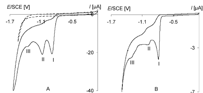
Figure 1. Cyclic voltammograms at a glassy carbon electrode in acetate buffer/ethanol (1:1) (---) and in the presence of 9 (—) ( C = 10^{-3} \text{ mol L}^{-1} ) at a scan rate of 0.2 \text{ V s}^{-1} (A) and 2 \times 10^{-3} \text{ V s}^{-1} (B).
