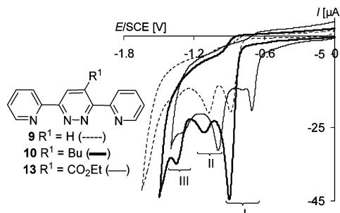
Figure 2. Cyclic voltammograms at a glassy carbon electrode in acetate buffer/ethanol (1:1) of compounds 9 (---), 10 (—), and 13 (—) ( C = 10^{-3}\text{ mol L}^{-1} ) at a scan rate of 0.2\text{ V s}^{-1} .
