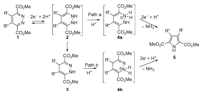
Scheme 1. Mechanism for the electrochemical reduction of bis(methoxycarbonyl)pyridazines.
