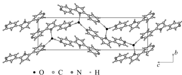
Figure 7. ORTEP diagram of dipyridin-4-ylpyrrole 23 .
